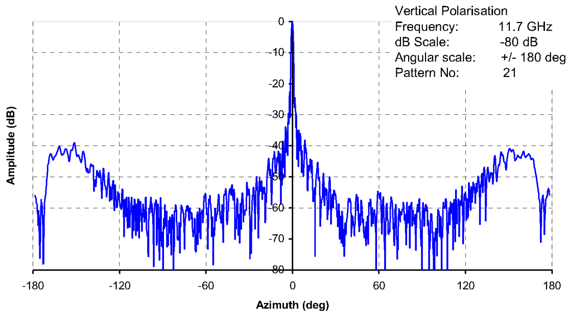
1.5m Solid Data File: Adv11
